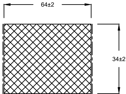
SECTION AT 'XX'
